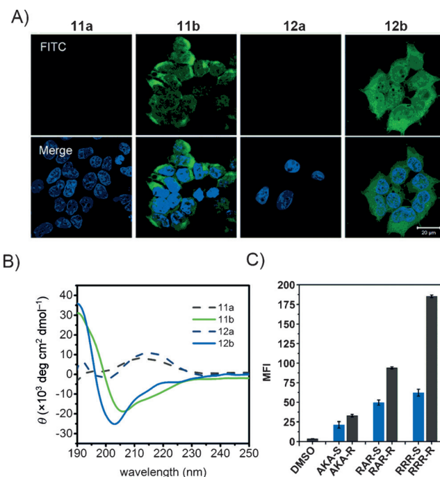
Figure 4. Cell permeability of pentapeptide diastereomers. A) Fluorescent confocal microscopy images of HEK293T cells incubated with FITC labeled peptides 11a/b and 12a/b (5 \mu M) at 37 °C for 2 h (blue (DAPI), green (FITC)). B) CD spectra of peptides 11a/b and 12a/b at 20 °C in 50% TFE buffer. C) Flow cytometry measurements of HEK293T cells with peptide 11a/b , 12a/b , and 13a/b (5 \mu M) at 37 °C for 2 h.
